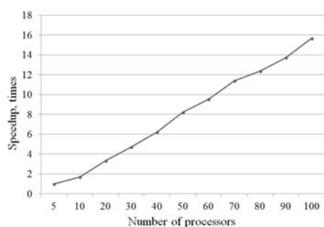
Fig. 1. Speedup depending on the number of processors
