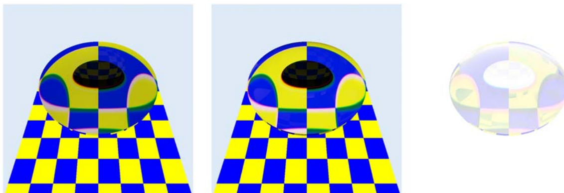
Figure 4. Images from left to right: calculation on the basis of Schlick approximation, calculation by Fresnel, negative difference
